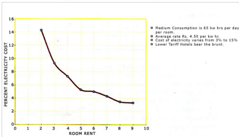
FIG 5 COST OF SPECIFIC CONSUMPTION V/S ROOM VENT
