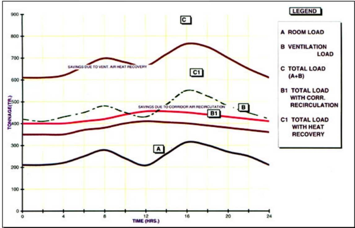
FIG 2 LOAD PROFILE - 550 ROOMS
