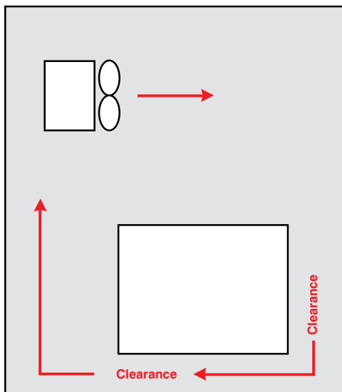
Figure 3 : For product holding applications, the unit cooler is placed so that the product, walls, and floor form a duct for the return air to travel around the product.
