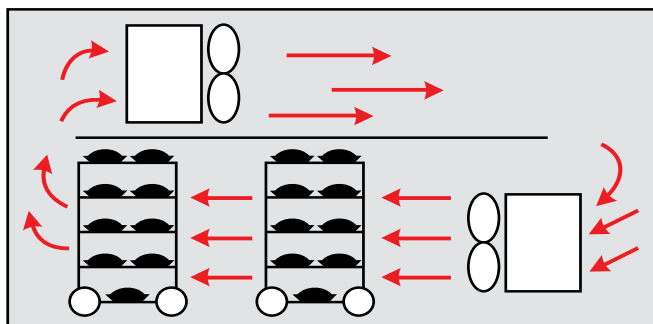
Figure 5 : Clearly defined return and discharge air streams result in peak unit cooler performance.
