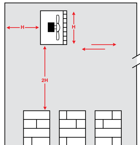
Figure 1 : Adequate clearances must be maintained on all sides of a unit cooler to ensure peak performance.
