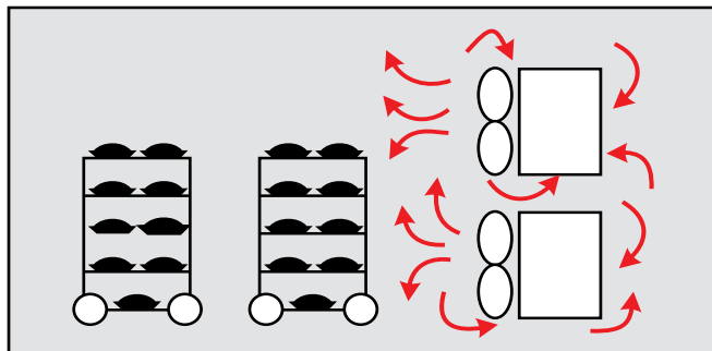
Figure 4 : Shortcycling of air around the unit coolers and poor distribution of air over the product are problems associated with blast cooling or freezing.
