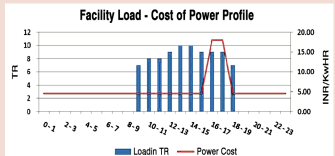
Figure 7: Load and power cost profile
