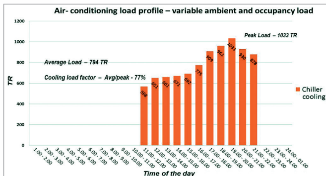
Figure 10: HVAC requirement in Option 1
