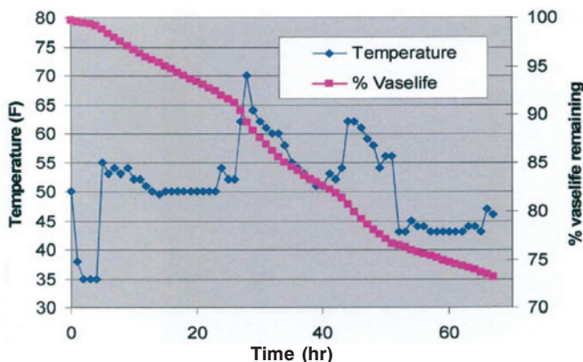
Figure 1 : Effect of poor temperature control on vase life of flowers 6
