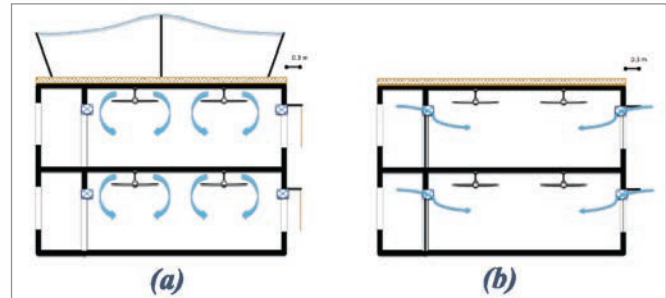
Figure 4: Schematic representation of Package 1, with retrofitted single glazing, roof insulation, integrated window purifying ventilators, bamboo window shading, and summer canopy (a) in summer (b) in winter
