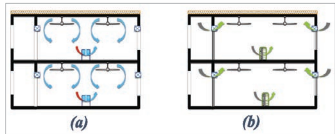
Figure 5.: Schematic representation of Package 2, with fully operable double-glazed windows, roof insulation, integrated window purifying ventilators, and modular electrostatic precipitator/evaporative cooling (a) in summer (b) in winter
