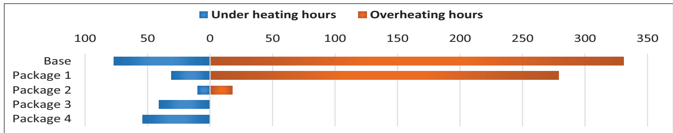
Figure 9: Thermal performance of the different packages in the classroom at the ground floor, expressed in under- and over-heating hours outside the 80% satisfaction range of the ATC model with a total amount of occupancy hours = 1890 h
