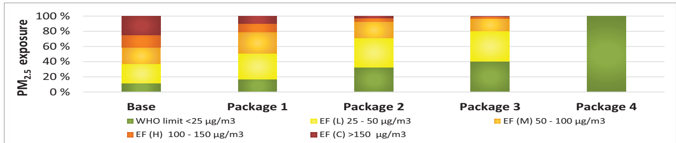
Figure 8: Annual mean indoor PM 2.5 exposure categorized in exceedance factor (EF) hours - Low (L), Moderate (M), High (H), and Critical (C) - and hours underneath daily WHO limit, over in total 1890 occupancy hours
