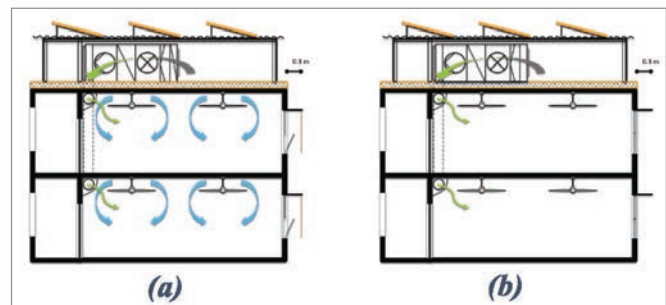
Figure 7: Schematic representation of Package 4, with partly operable double-glazed windows, roof insulation, air handling unit with three stage air filtering and cooling coil, and solar PV (a) in summer (b) in winter
