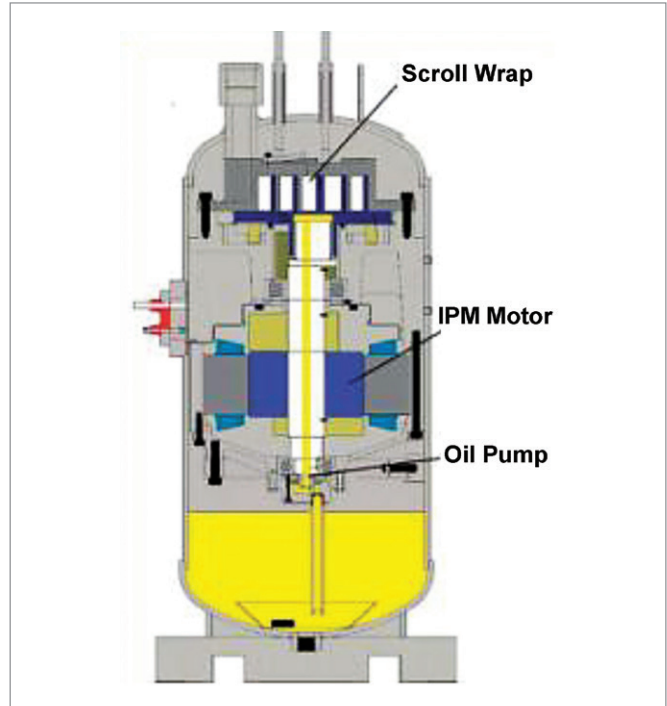
Figure 2: Semi-hermetic ammonia scroll compressor
