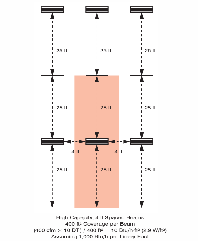
Figure 5: High capacity beams.
