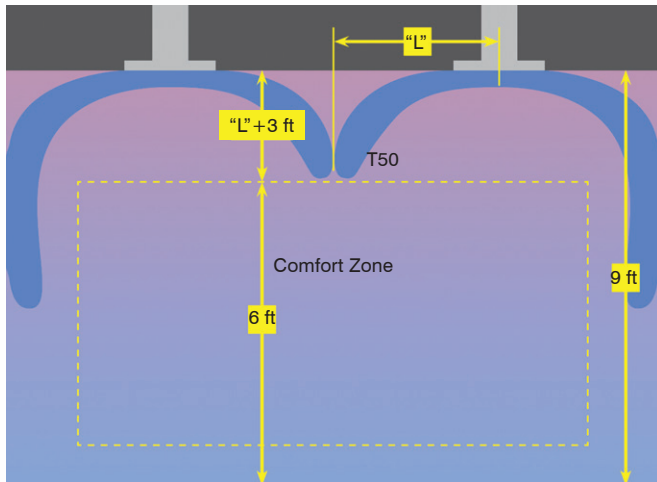
Figure 1: Jet collision.
