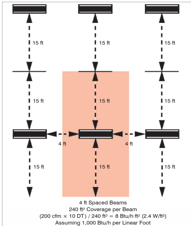
Figure 2: Four foot spaced beams.
