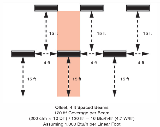
Figure 4: Staggered beams.
