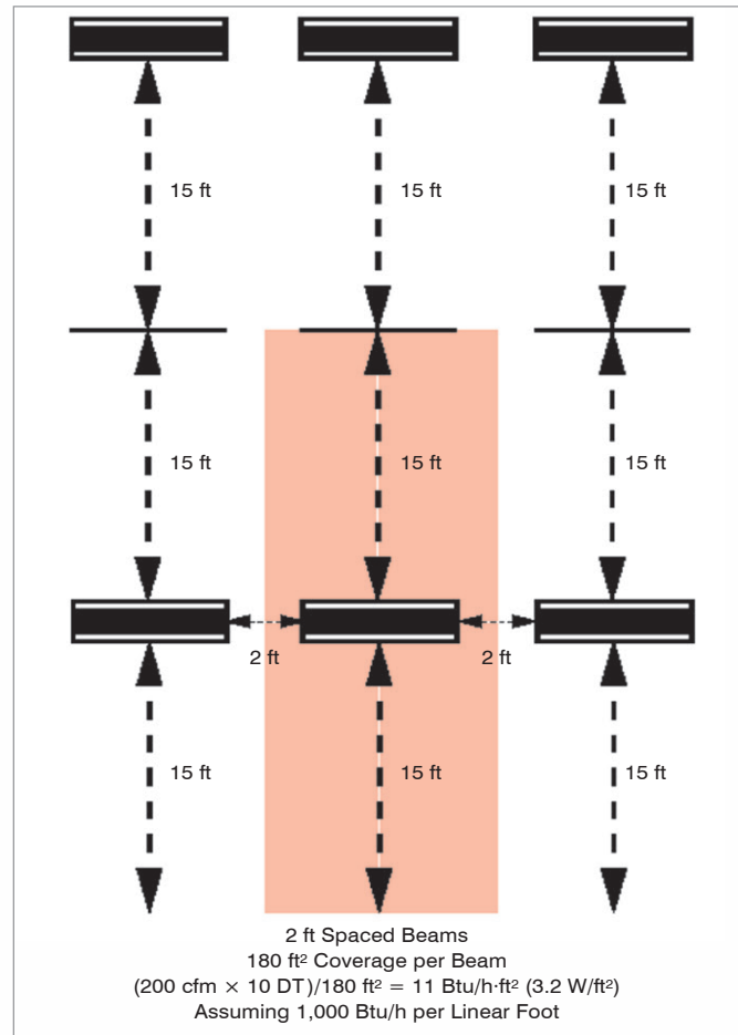
Figure 3: Two foot spaced beams.
