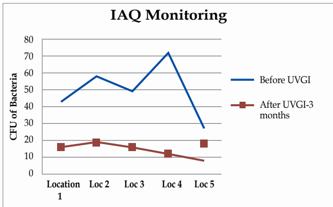
Figure 4: IAQ after installation of UVGI units
