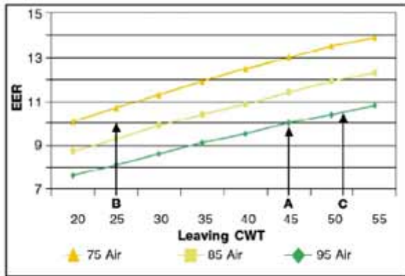
Figure 3 : EER of air-cooled chillers (includes heat rejection)
