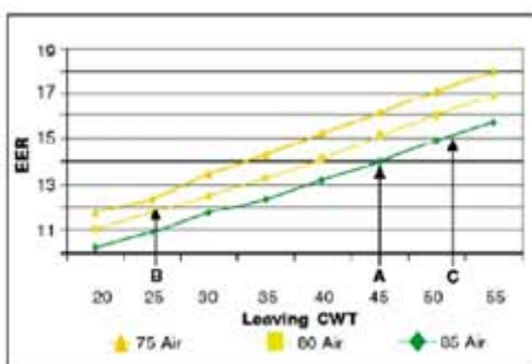
Figure 4 : Water-cooled chiller (comp. only)
