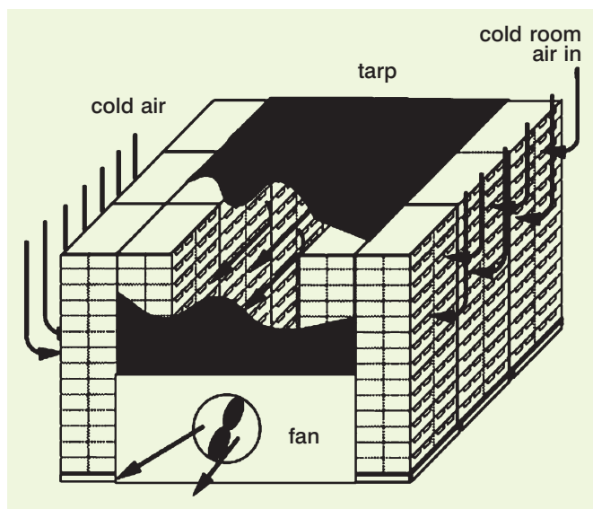
Figure 2: Schematic of a tunnel-type precooler
