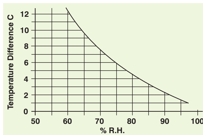
Figure 4: Approximate relative humidity (0°- +2°C room only) Courtesy of Buffalo Trident, a division of Bitzer, Australia.
