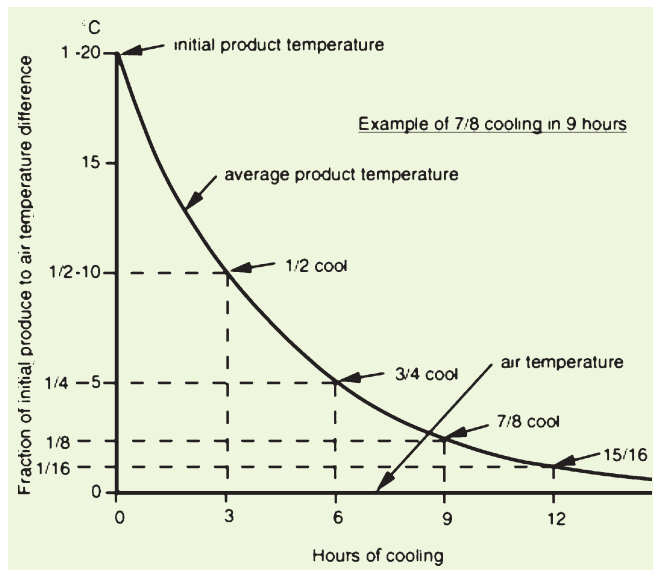
Figure 3: Typical time-temperature pattern in produce cooling. Numbers along the temperature curve indicate the fraction obtained by dividing the difference between product temperature and air temperature in the cooler by the difference between the initial produce temperature and the air temperature.
