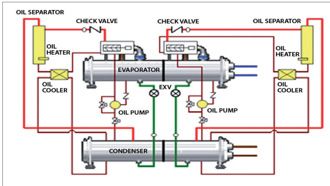
Figure 2: Typical water cooled screw chiller
