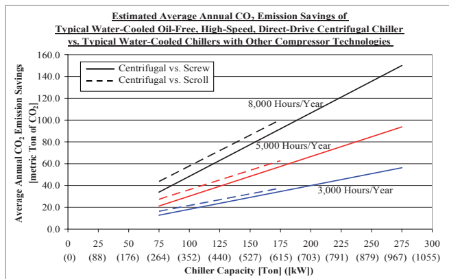
Figure 10: Estimated average annual CO 2 emission savings [metric Ton of CO 2 ]
