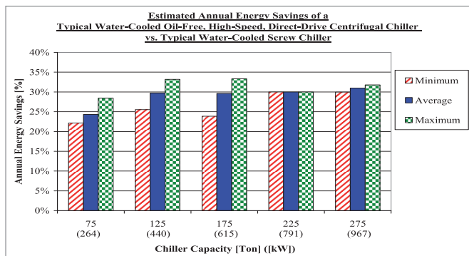
Figure 6: Estimated annual energy savings compared to typical water cooled screw chiller
