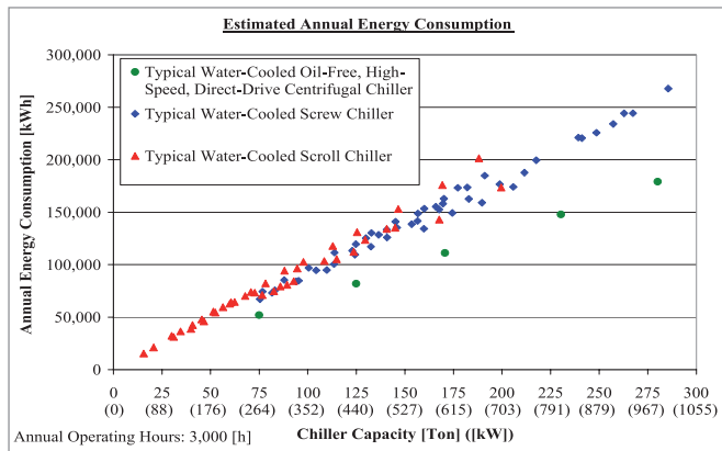
Figure 5: Estimated annual energy consumption
