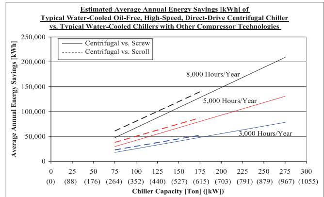
Figure 8: Estimated average annual energy savings [kWh]
