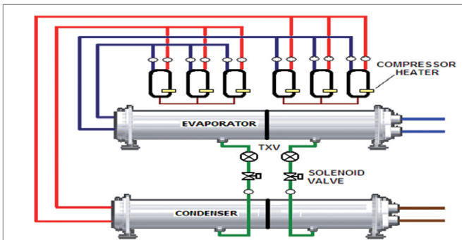
Figure 3: Typical water cooled scroll chiller
