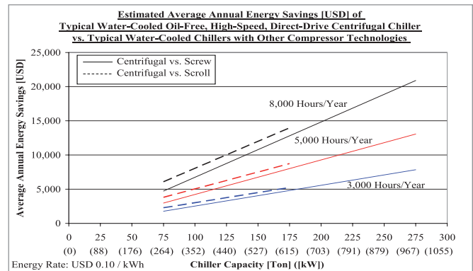
Figure 9: Estimated average annual energy savings [USD]
