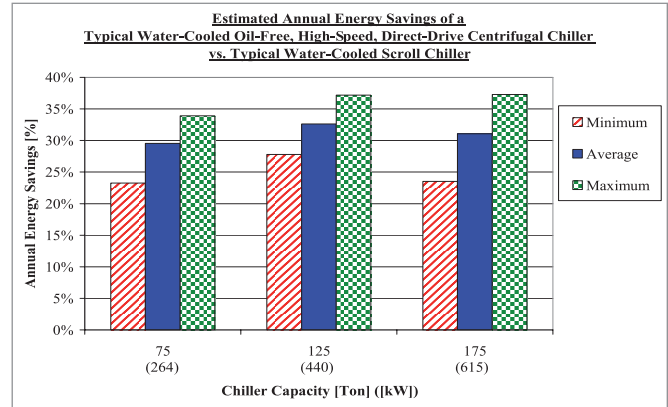
Figure 7: Estimated annual energy savings compared to typical water-cooled scroll chiller
