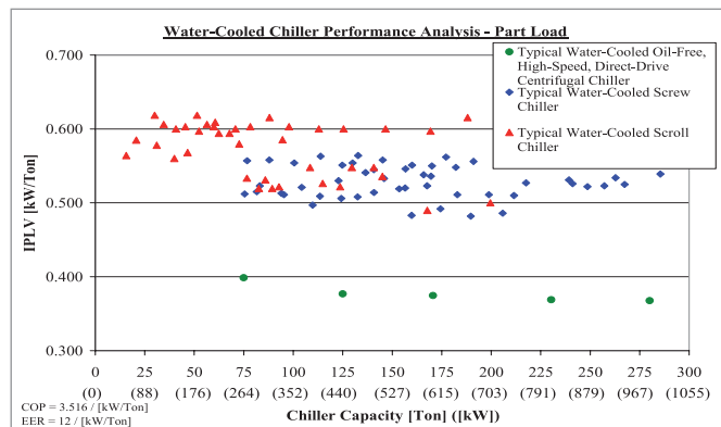
Figure 4: Typical water cooled chiller part load performance
