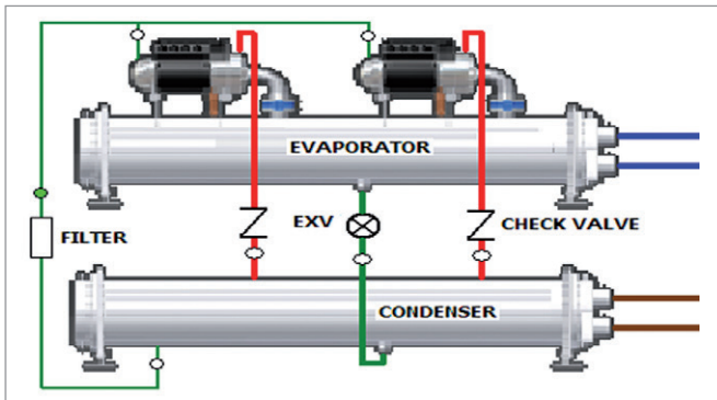
Figure 1: Typical water cooled oil-free, high speed, direct-drive centrifugal chiller
