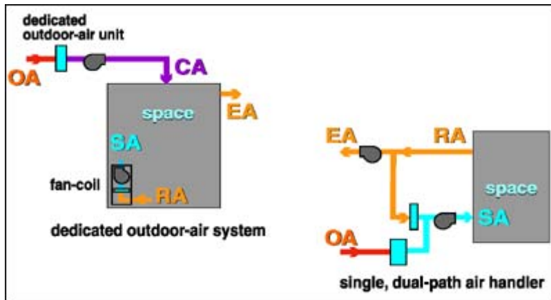
Figure 3 : CV systems with separate path for OA treatment
