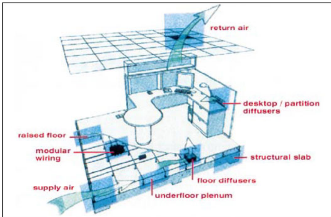
Figure 1 : Cutaway of typical office work space with underfloor air distribution.
